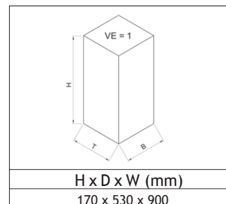
Pic.: Type console D, galvanized, Art.-No. 1092
