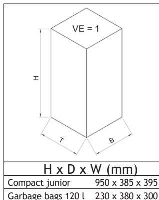
Pic.: Compact junior, hot galvanized, Art.-No. 1001
