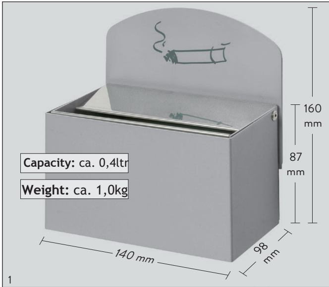
Wall ashtray WH9, silver with plate and labels, Art.-Nr. 14761
